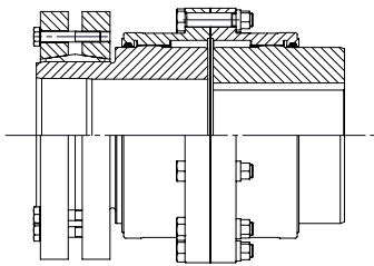
EXTERNAL CLAMPING
