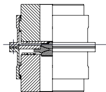
FSV/FSUSVA STANDARD VERTICAL WITH AXIAL LOAD C4195a + C4196a Page 34 & 35
