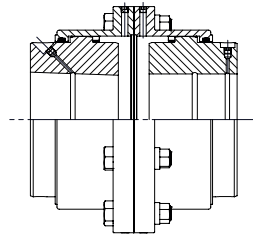
INTERFERENCE FIT
