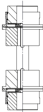
FLOATING SHAFT VERTICAL WITH AXIAL LOAD
