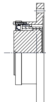
FLYWHEEL ADAPTER
