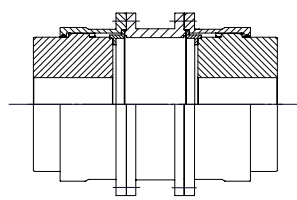
FSELE/FSUSELE SPACER EXECUTION, LIMITED END FLOAT C4200a Page 41
